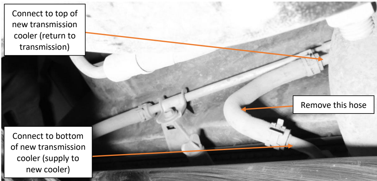
Stock transmission cooler lines running to factory cooler in radiator bottom tank.
