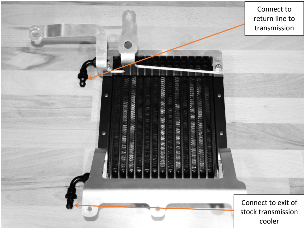
Cooler Assembly Hose Connections
