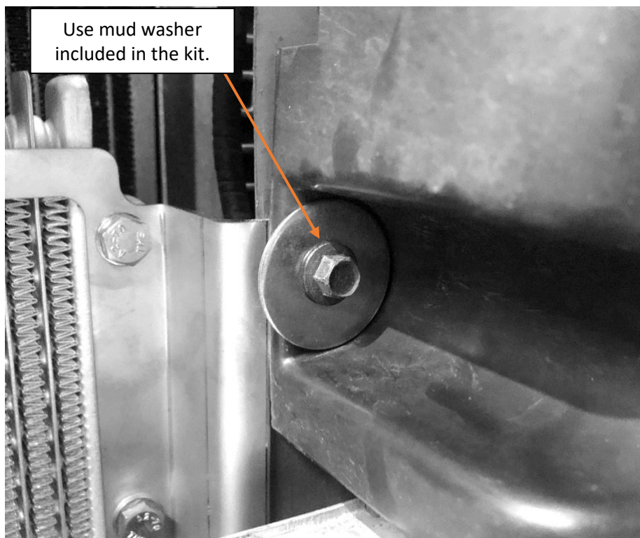
The top bolt installed with trim piece also secures the top outer mount for transmission cooler bracket.
