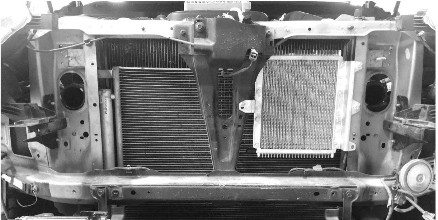
Transmission Cooler Assembly Bolted in Place. Note: Cooler sits on back face of the bracket, with nuts towards the rear, bolts to the front. The inlet and outlet ports should be facing the center support of the vehicle. Note there are only two bolts needed to secure the cooler bracket to the vehicle at this stage, the top bolt is reused when the factory end trim pieces are reinstalled.
