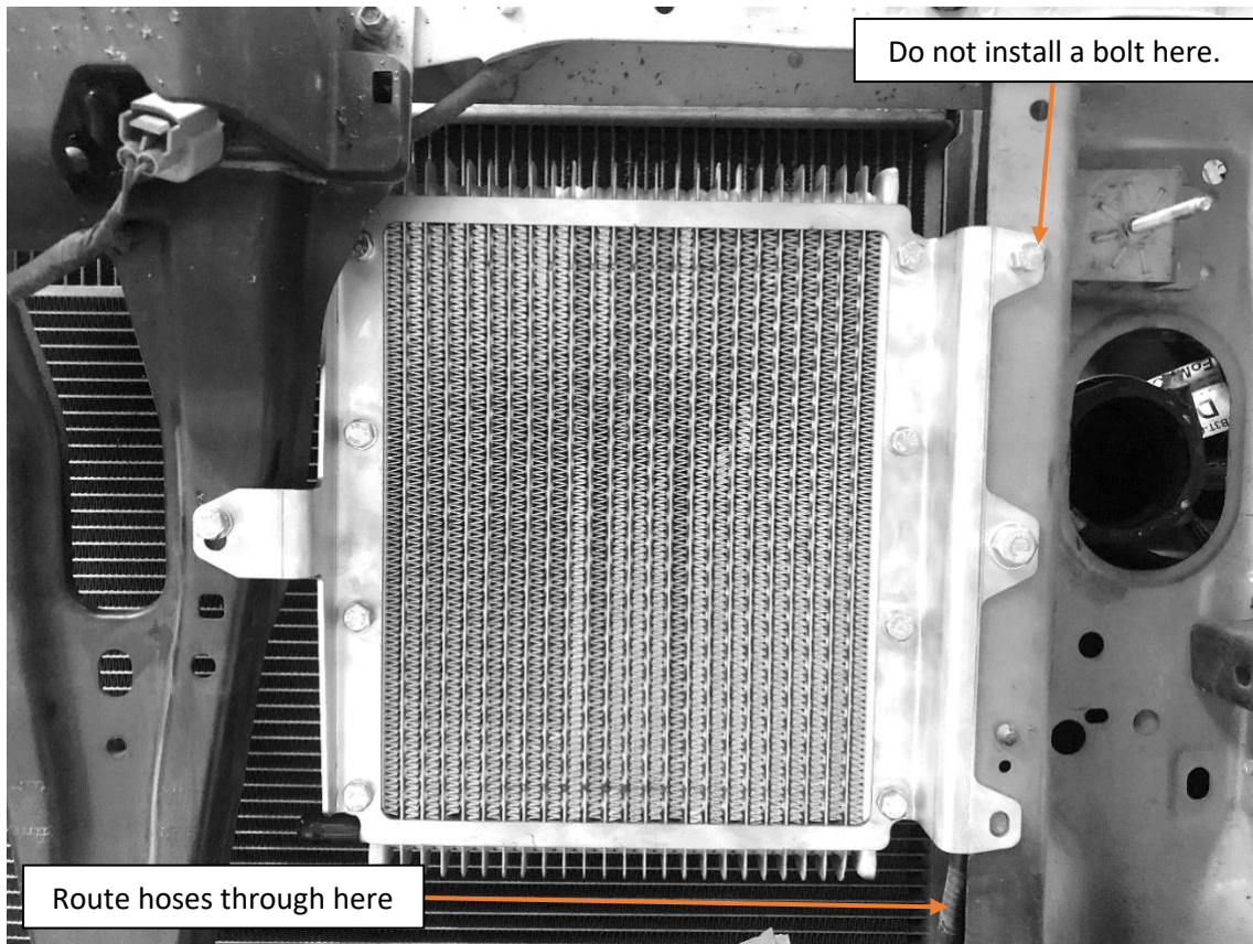
Transmission cooler installed – closeup.
