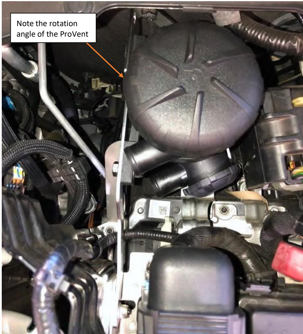
ProVent 200 bolted into place at correct rotation, 25-19mm reducers and elbows are shown installed in this image to give you an idea of fitment (clamps not fitted)
