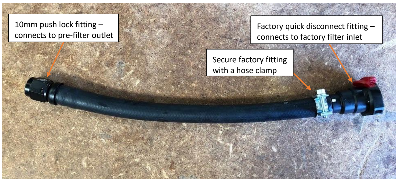
hose construction from pre-filter outlet to factory filter inlet
